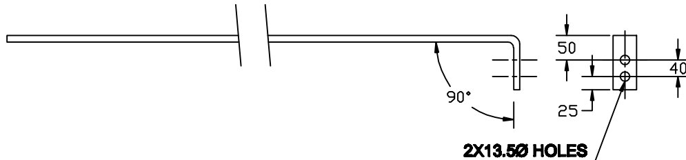
DETAIL OF FLAT TYPE 'D'
