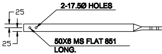
DETAILS OF FLAT TYPE 'C'
